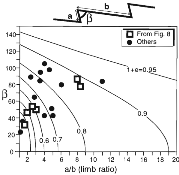
Fig. 14. Long limb over short limb ratio of large-scale folds in the Bergsdalen Nappe plotted against their opening (interlimb) angle \beta . Points represent individual measurements of continuous, large-scale (>100 m long) folds from constructed map profiles. Contours of constant shortening of the folded layer have been estimated (see Appendix), using the simplification that the folds have angular hinges. Note that this gives a minimum estimate of the shortening since layer-parallel shortening has been neglected. No systematic relationship between the amount of shortening and position in the décollement zone has been identified from the data.
