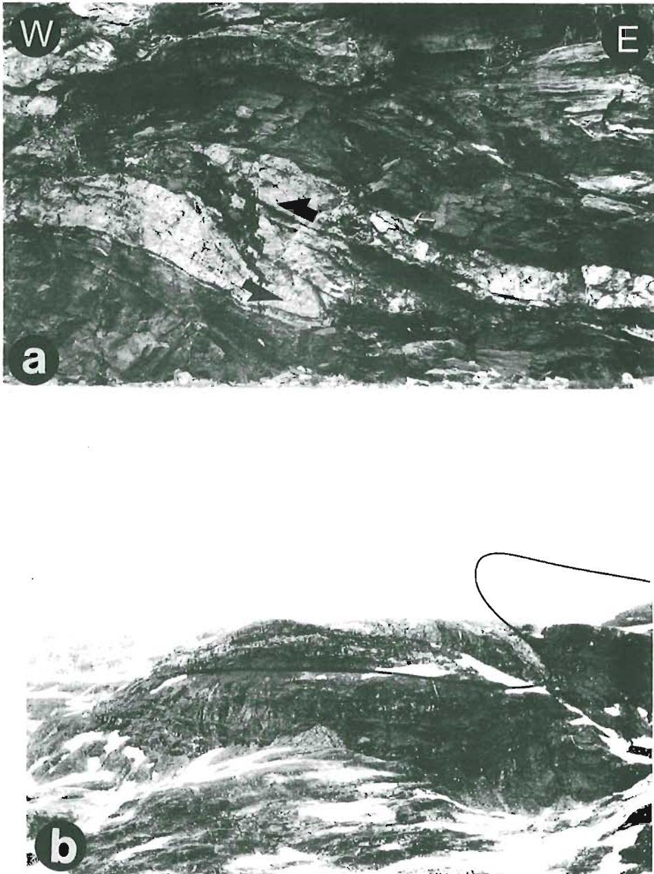
Fig. 7. (a) Thrust-like structure indicating shortening of the light granitic dike in the dark biotite gneiss, Lower Bergsdalen Nappe (Eikedalen). (Note fold hinge preserved to the right of the lower arrow.) The width of the photograph is about 10 m. (b) Large-scale fold in the Upper Bergsdalen Nappe, looking NNE. The cliff is about 200 m high.
