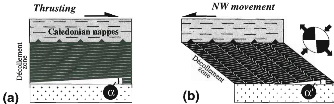
Fig. 1. A shear zone with an internal layering initially inclined to the boundaries as shown in (a) is likely to result in the development of asymmetric folds with a vergence corresponding to the sense of shear (b). This schematic illustration can be thought of as a vertical NW-SE section through the décollement zone during (a) thrusting ( D_1 ) and (b) back movement ( D_2 ). The planar fabric and lithological layering in the décollement zone made an acute angle ( \alpha ) with the shear zone at the end of the thrusting. This geometry explains the widespread formation of folds or reverse-slip crenulations during D_2 (b). The orientation of the incremental strain ellipse is indicated in (b).
