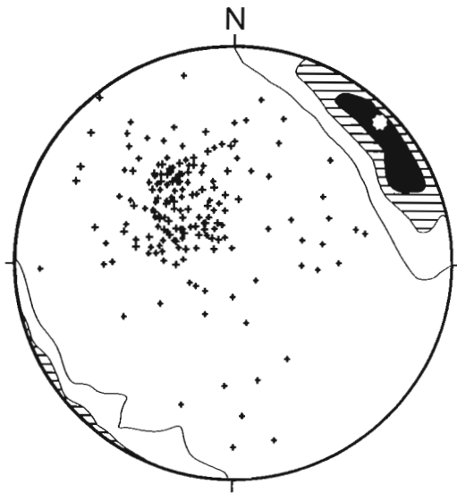
Fig. 6. Equal-area projection of 850 F_2 hinge lines. Contour interval = 2%/1% area. The maximum principal axis of the Bingham distribution of the data set is indicated (046/6). Individual points are poles to related axial surface foliations. Data from southwest Norway, mostly from the Bergsdalen Nappes.
