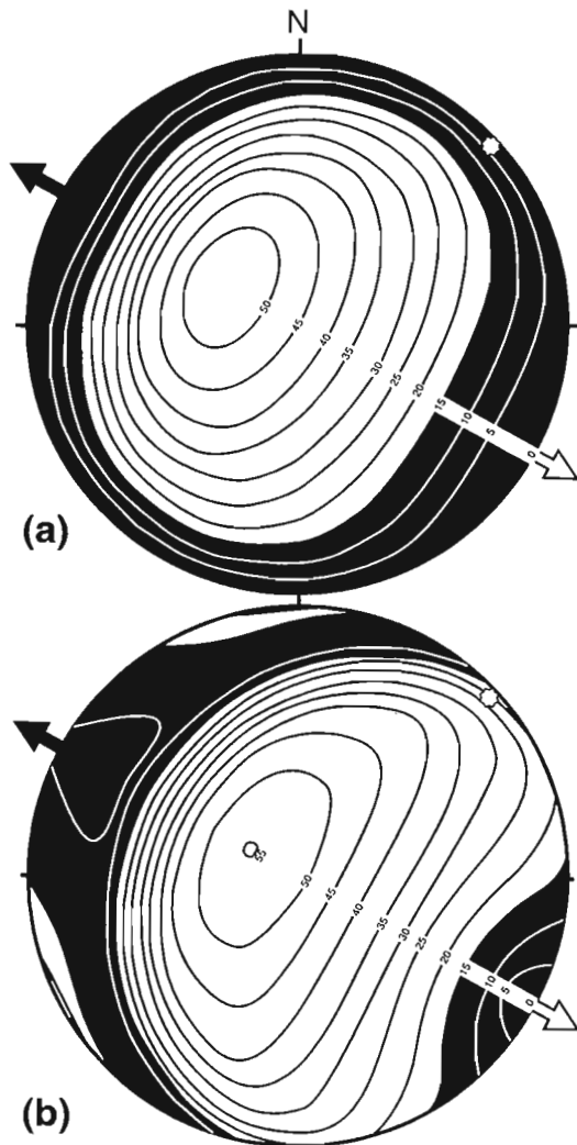
Fig. 11. (a) Stereonet (equal area) with contours that shows how much a given line will rotate for (a) a simple shear with \gamma = 1 (horizontal shear plane with shear direction to the northwest), and (b) the same deformation with an additional, simultaneous pure shear component (vertical shortening and stretching in the shear direction) so that the kinematic vorticity number is 0.8. Area in black illustrates area of low rotation (rotation < 20^\circ ). Note how the low-rotation belt around the horizontal shear plane in (a) is changed in the presence of a pure shear (b). The maximum point of concentration of hinge lines from the Bergsdalen Nappes (Fig. 6) is indicated in both plots (corrected for the non-horizontal orientation of the décollement zone in this area), and shows how an additional pure shear implies a larger rotation of hinge lines with this orientation.
