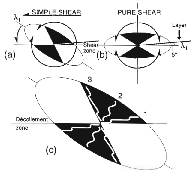
Fig. 12. Strain ellipse after an increment of (a) simple shearing ( \gamma = 1 ) and (b) a corresponding strain produced by pure shearing. Black field indicate area of finite shortening. Arrows indicate direction of line rotation. Note that a gently WNW-dipping line (plane) that makes a low angle with the shear plane is in the shortening field for simple shear and rotates sympathetically with the sense of shearing, whereas for pure shearing a similarly orientated line undergoes extension and the opposite sense of rotation. (c) Strain ellipse in (a) showing how vergence depend on initial orientation of the folded layer. The Type 1 style is the one observed in the field, supporting the idea that the Caledonian planar fabric was dipping slightly more to the west-north-west than did the décollement (shear) zone at the onset of the back movement ( D_2 ).
